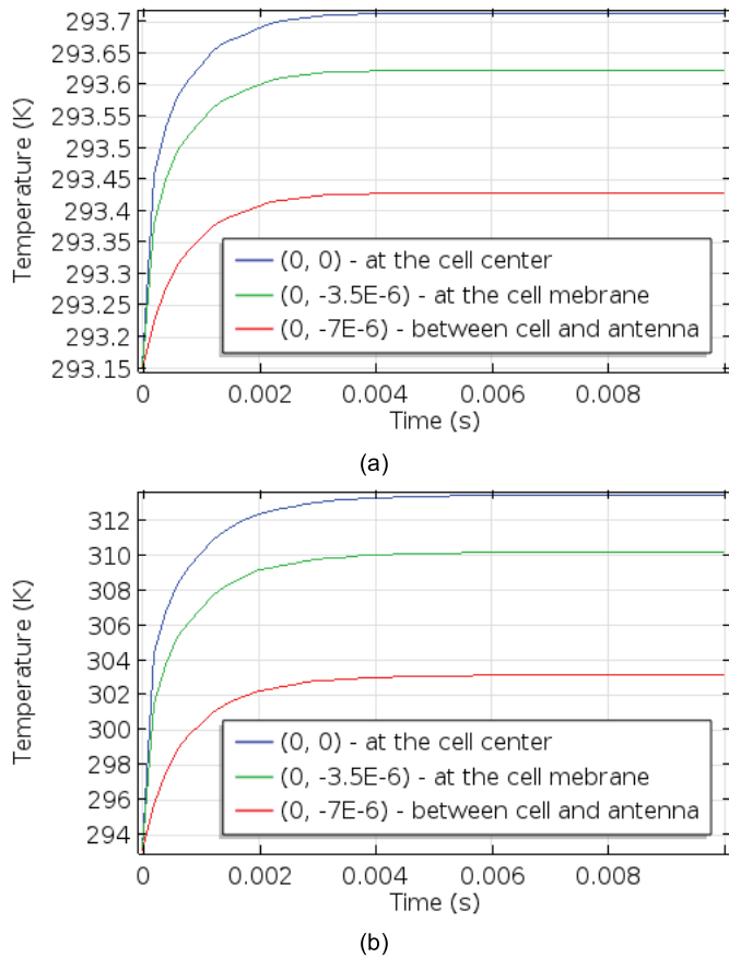
Fig. 6. The temperature variation as a function of time experienced at the cell center, at the cell membrane and between the cell and the antenna for a heating time of 10 ms and a dipole moment of (a) 1 mA · m and (b) 6 mA · m.
