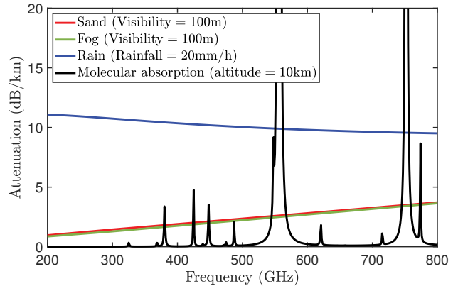
Fig. 3. Attenuation versus frequency for the different weather conditions.
