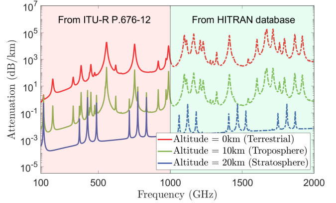
Fig. 4. The molecular absorption loss versus frequency with altitude at 0 km, 10 km, and 20 km, corresponding to the terrestrial communication, troposphere and stratosphere in summer and high latitude region.
