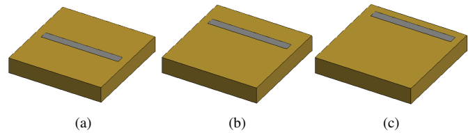
Fig. 5. Different positions of the graphene patch with respect to the substrate: patch in the center of the substrate (a), at 1.25 \mu\text{m} from the center (b) and at 2.5 \mu\text{m} from the center (c).
