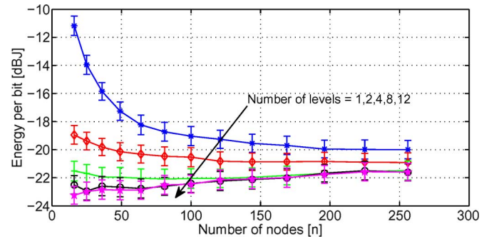
Fig. 8. Energy per bit consumption for a varying number of power levels. Center frequency and bandwidth are chosen optimally; FBR is used. The error bars represent the uncertainty interval at the 95% confidence level.
