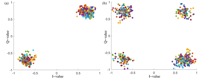
Fig. 2. Software processed output constellations for (a) channel-1 (BPSK modulated data symbols, error vector magnitude [EVM]: -19.5 dB), (b) channel-2 (QPSK-modulated data symbols, EVM: -17.2 dB).
