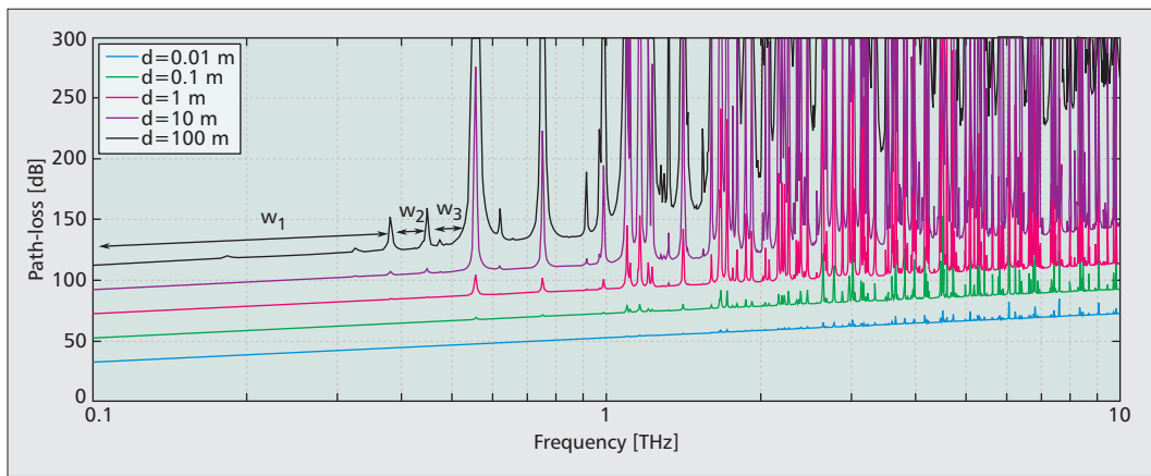
Figure 2. Path loss in the THz Band for different transmission distances.
