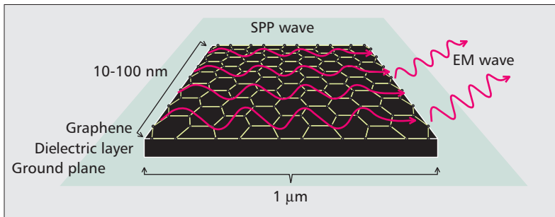
Figure 1. A graphene-based plasmonic THz Band antenna [10].
