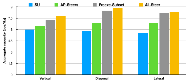
Fig. 8: Average aggregate capacity for different user groups
