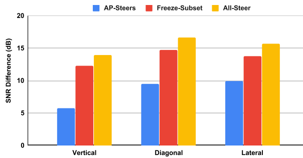
Fig. 9. Received SNR difference for different user groups.
