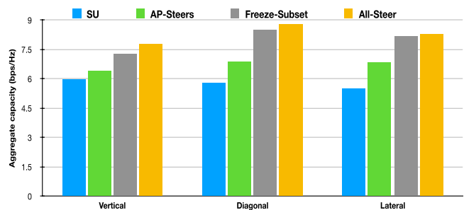
Fig. 8. Average aggregate capacity for different user groups.
