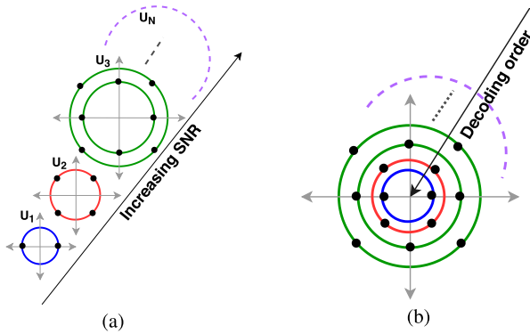
Fig. 3. (a) Multi-user Overlaid APSK constellations showing users with constellation rings of increasing radius. (b) SNR based SIC decoding order.
