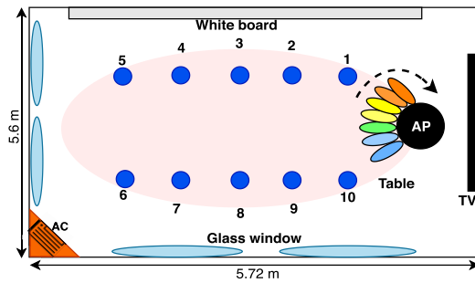
Fig. 13. Experimental floor plan used for measurement of data using WARP-60 testbed.
