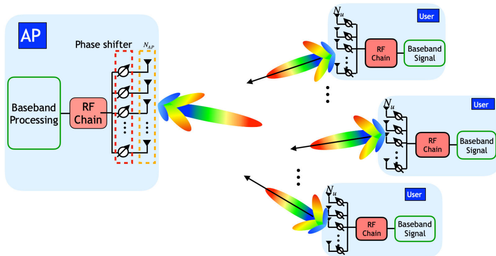
Fig. 1. AP with single RF chain system supporting multiple users on the uplink.
