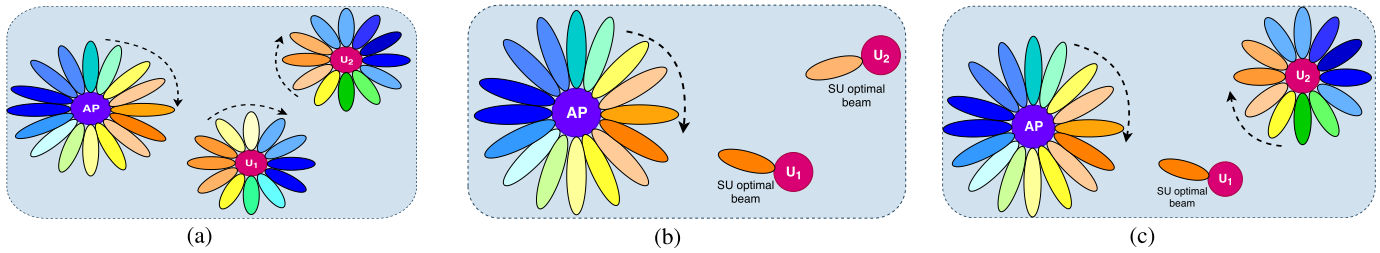
Fig. 5. Illustrative scenario of constrained beam adaptation using (a) All-Steer . (b) AP-Steers . (c) Freeze-Subset .
