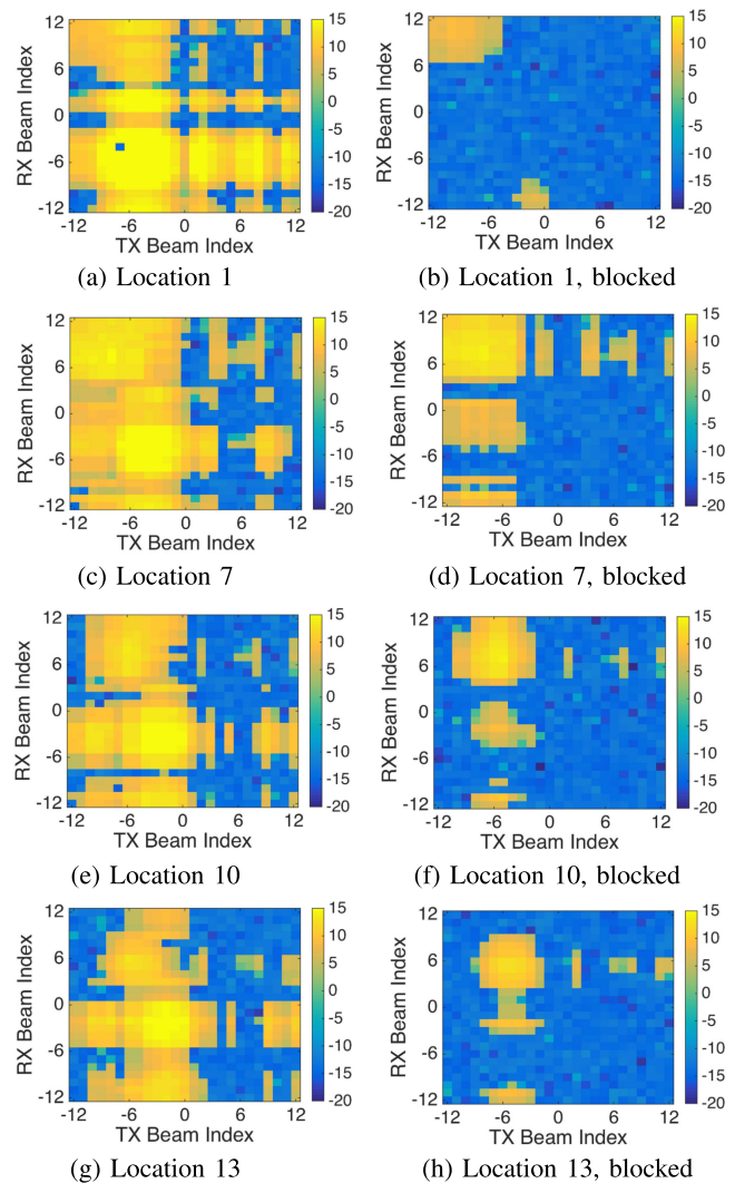
Fig. 11. SNR heatmaps for all beam pair combinations for user location indices 1, 7, 10 and 13 in the lobby under LOS connectivity (left column) and blockage (right column).
