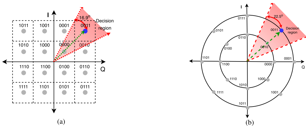
Fig. 4. Comparison of maximum angle error tolerance for symbol '0011' sent using (a) 16-QAM. (b) 16-APSK.
