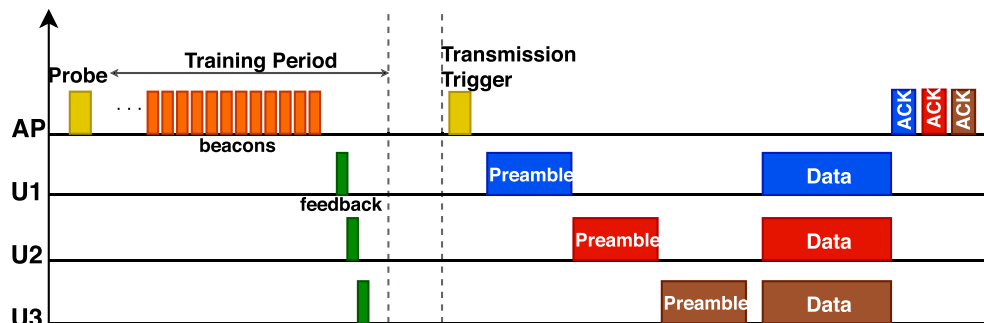
Fig. 2. Different stages of UMBRA timeline model.
