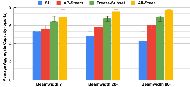
Fig. 14. Average of the aggregate capacity for all the users in the setup.
