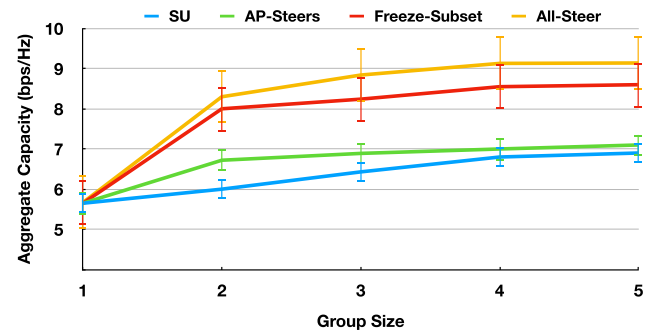
Fig. 15. Achievable Aggregate Capacity vs. Group Size.
