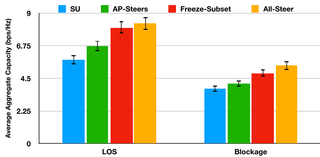
Fig. 12. Achievable Aggregate Rate under LOS Connectivity and Blockage.
